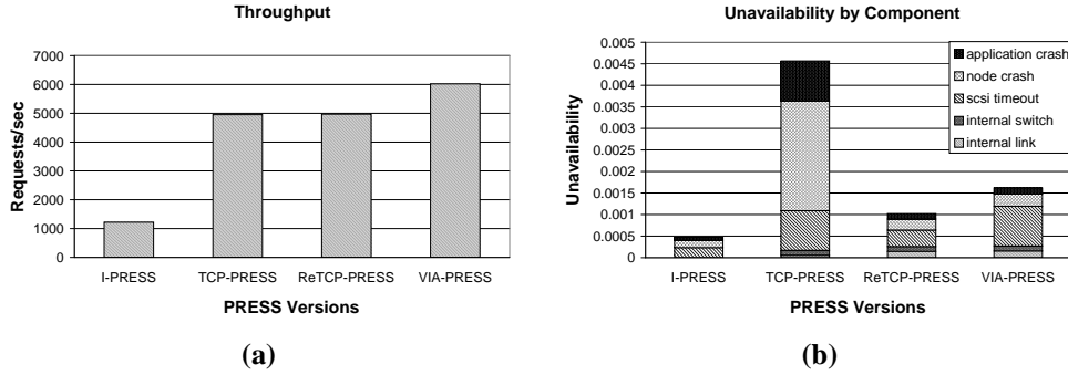
Figure 6: (a) Average modeled throughput and (b) modeled unavailability (1 - availability).
